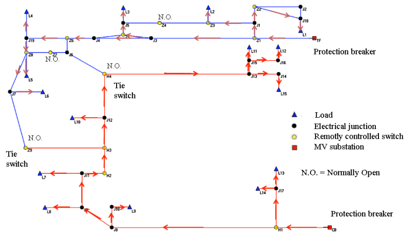
Fig. 2. A simplified view of MV power grid
