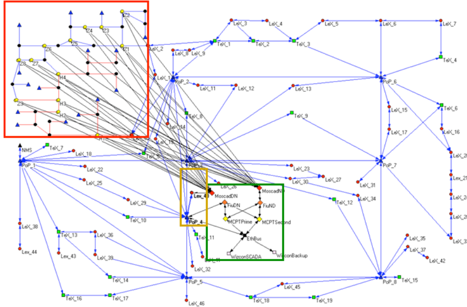
Fig. 4. Heterogeneous network supporting FISR service
